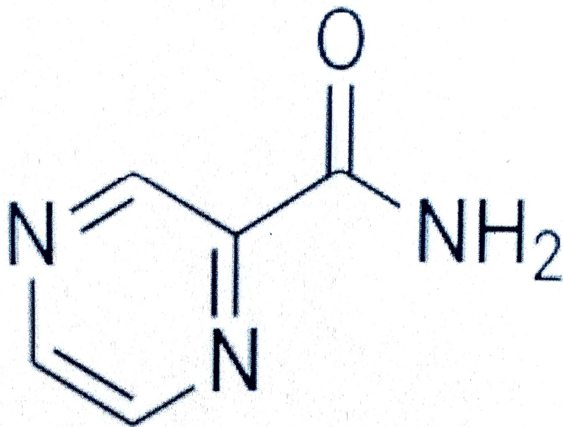
Pyrazinamide
