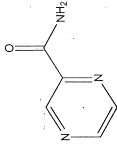
pyrazinamide
