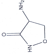
Cycloserine
