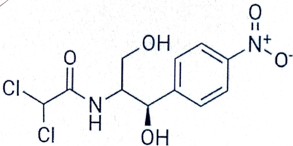
Chloramphenicol
