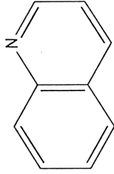
quinoline
