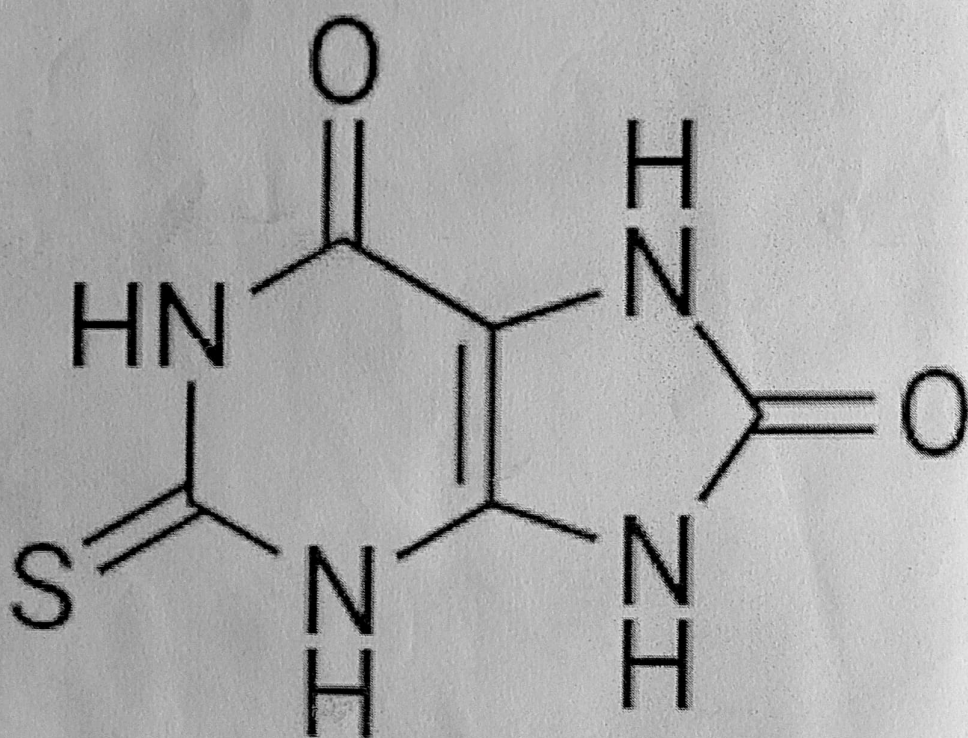
Thiouric acid
