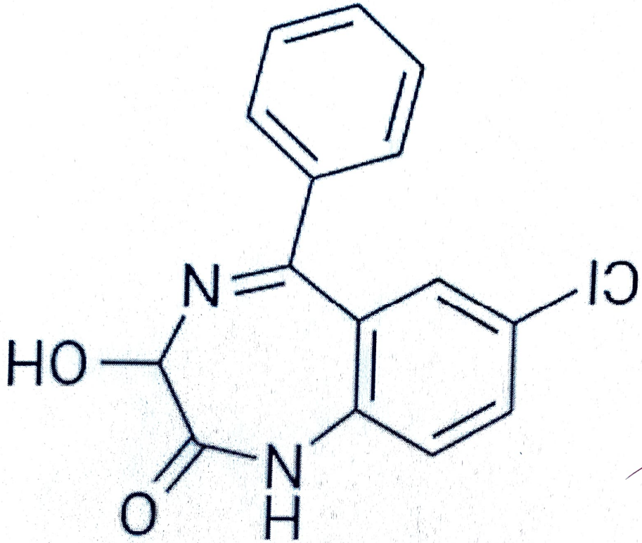
Oxazepam
