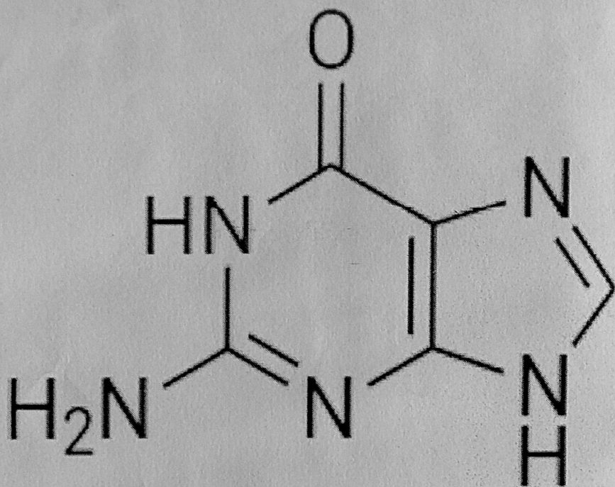
Guanine
